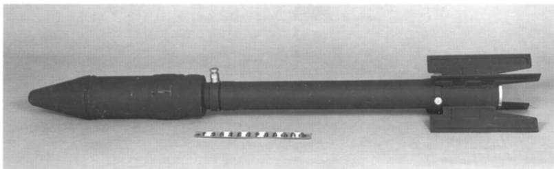
Figure C-19. Fin-stabilized rocket, 132-millimeter.
