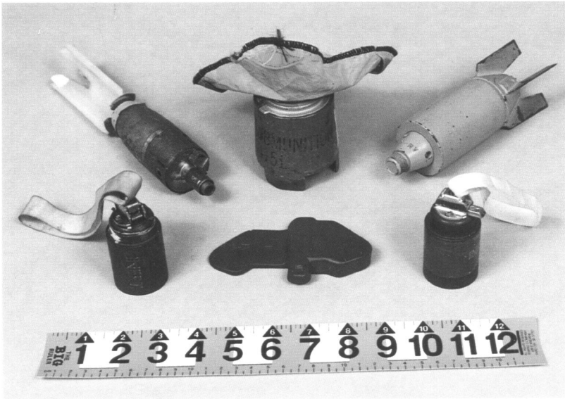
Figure B-7. APERS/AMAT submunitions (conventional).
