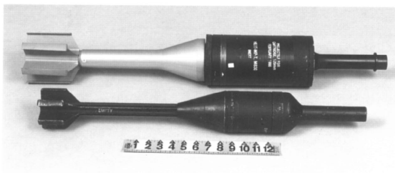
Figure C-7. Fin-stabilized projectiles, 90-millimeter (front) and 120-millimeter high-explosive antitank (HEAT) (rear).
