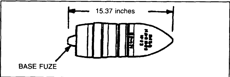
Figure 2-21. Base-fuzed projectile.
