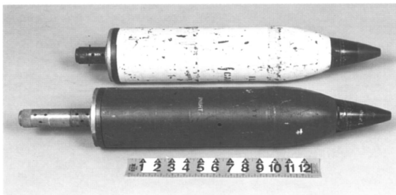
Figure C-12. Fin-stabilized mortars, 81-millimeter and 120-millimeter.
