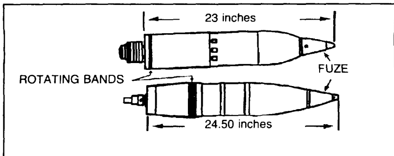
Figure 2-25. Spin-stabilized mortars.
