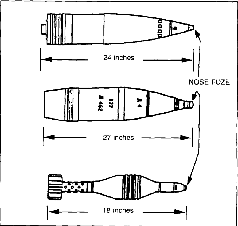
Figure 2-20. Nose-fuzed projectiles.
