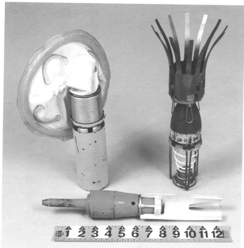
Figure B-8. AMAT/AT submunitions (conventional).
