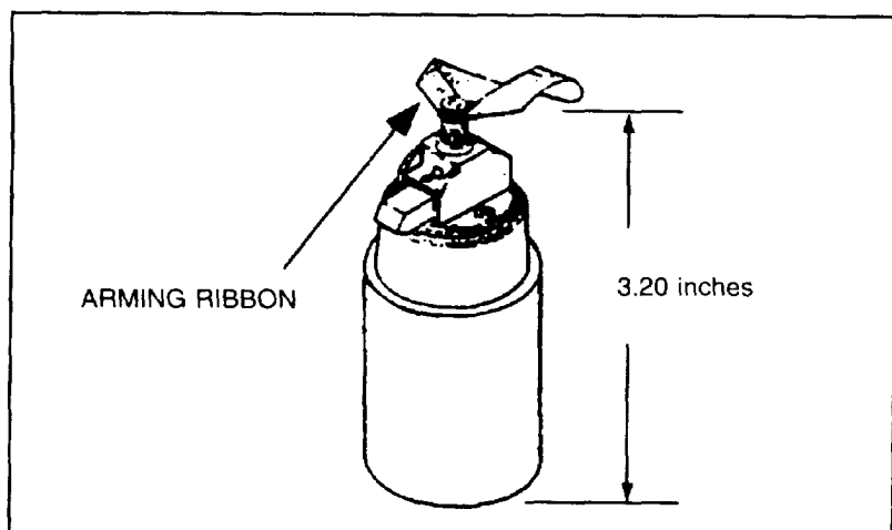
Figure 2-16. DP submunition.
